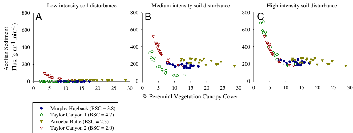
Fig. 5. Aeolian sediment flux following a 17.5 m s -1 wind event in relation to percent perennial vegetation canopy cover with low (A), medium (B), and high (C) intensity soil disturbances on four plots in dwarf Atriplex shrublands. Plots varied in perennial vegetation cover and average BSC development class (1, low; 6, high).
